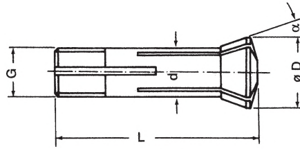
5C Collet
